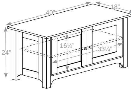
#2020 • 40W" 40"W x 18"D x 24"H 1 Adjustable shelf 2 doors
